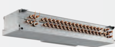
CMB-WM1016V-AA
